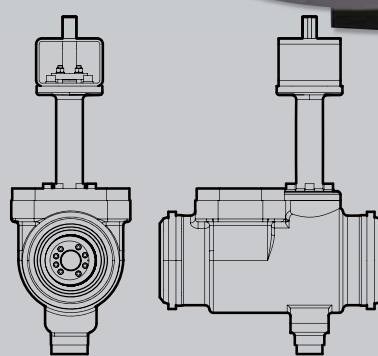
Side Entry Cryogenic Butt weld
