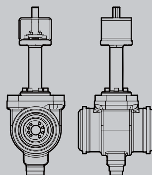
Top Entry Cryogenic Butt weld
